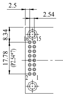
PIN DETAIL
